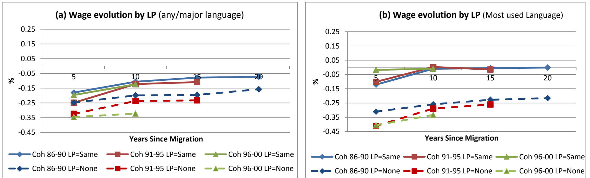
Figure 3. Immigrants' wage assimilation by Linguistic Proximity and arrival cohort (LP)
