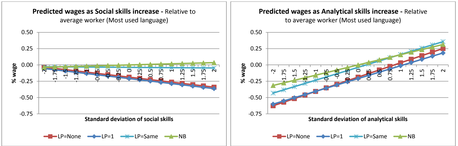
Figure 2. Predicted wages of immigrants in jobs requiring different skills (1) relative to average worker (wage=0)
