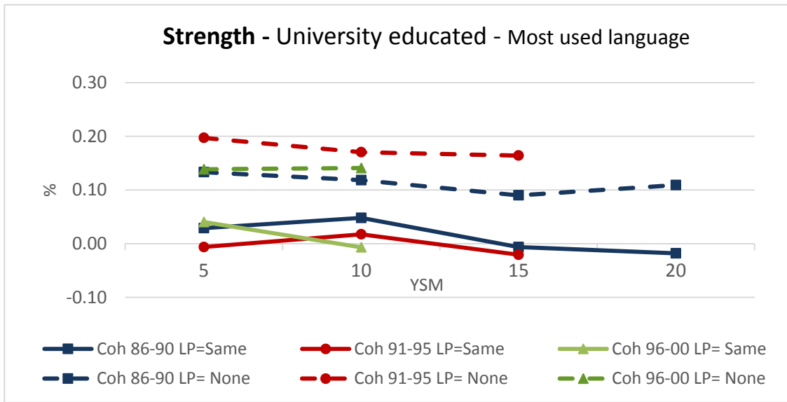
Figure 5. Evolution of job-required skills for university educated immigrants. By Linguistic Proximity and arrival cohort (Most used language)
