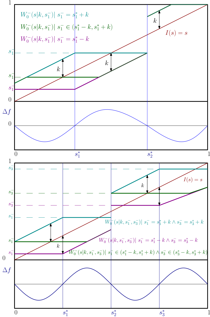
FIGURE 6. Potential W_0^-(s|k) 's for Two and Three Crossing Points
