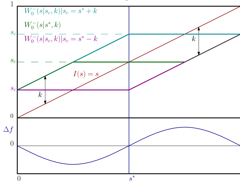
FIGURE 4. Three Potential W_0^-(s|k) 's, One Crossing Point
