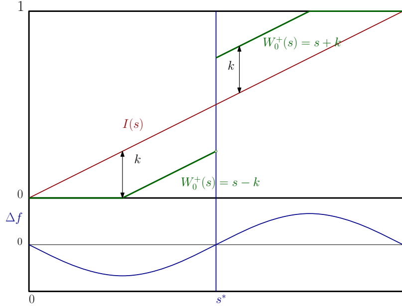
FIGURE 3. W_0^+(s|k) , One Crossing Point
